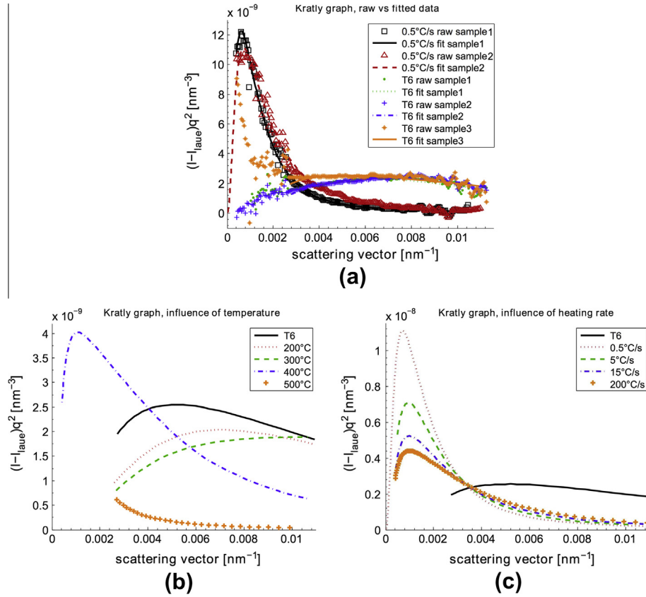
Fig. 2. (a) Comparison between three T6 samples and two samples heated at 0.5^\circ\text{C s}^{-1} . Raw and fitted data are represented. (b) One fitted data for each reached temperature treatment (c) One fitted data for each heating rate treatment.
