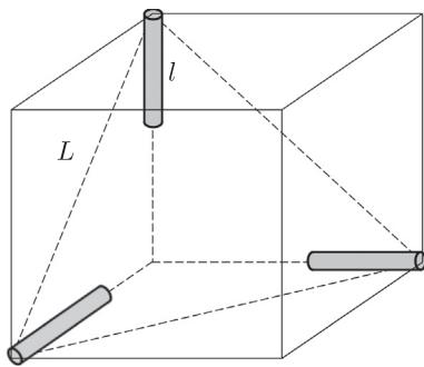
Fig. 8. Disposition of precipitates in the slip plane.
